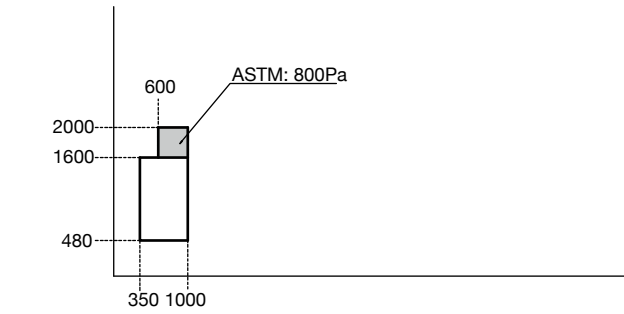
Casement Window (Multi Lock)
