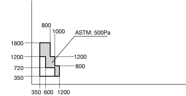
Casement Window (Single Lock)
