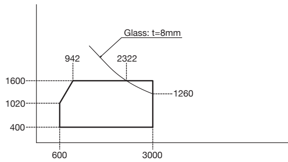
Sliding Window (3 panels on 2 tracks) SFS
