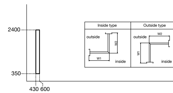
Casement Window (Single Lock)
