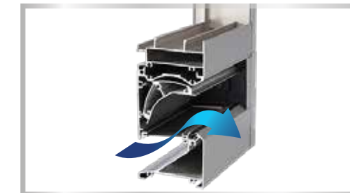
Smooth operation with bearing rollers
